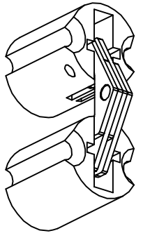
HINGE OPEN 180° ISOMETRIC VIEW
