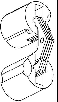
HINGE OPEN 180° ISOMETRIC VIEW
